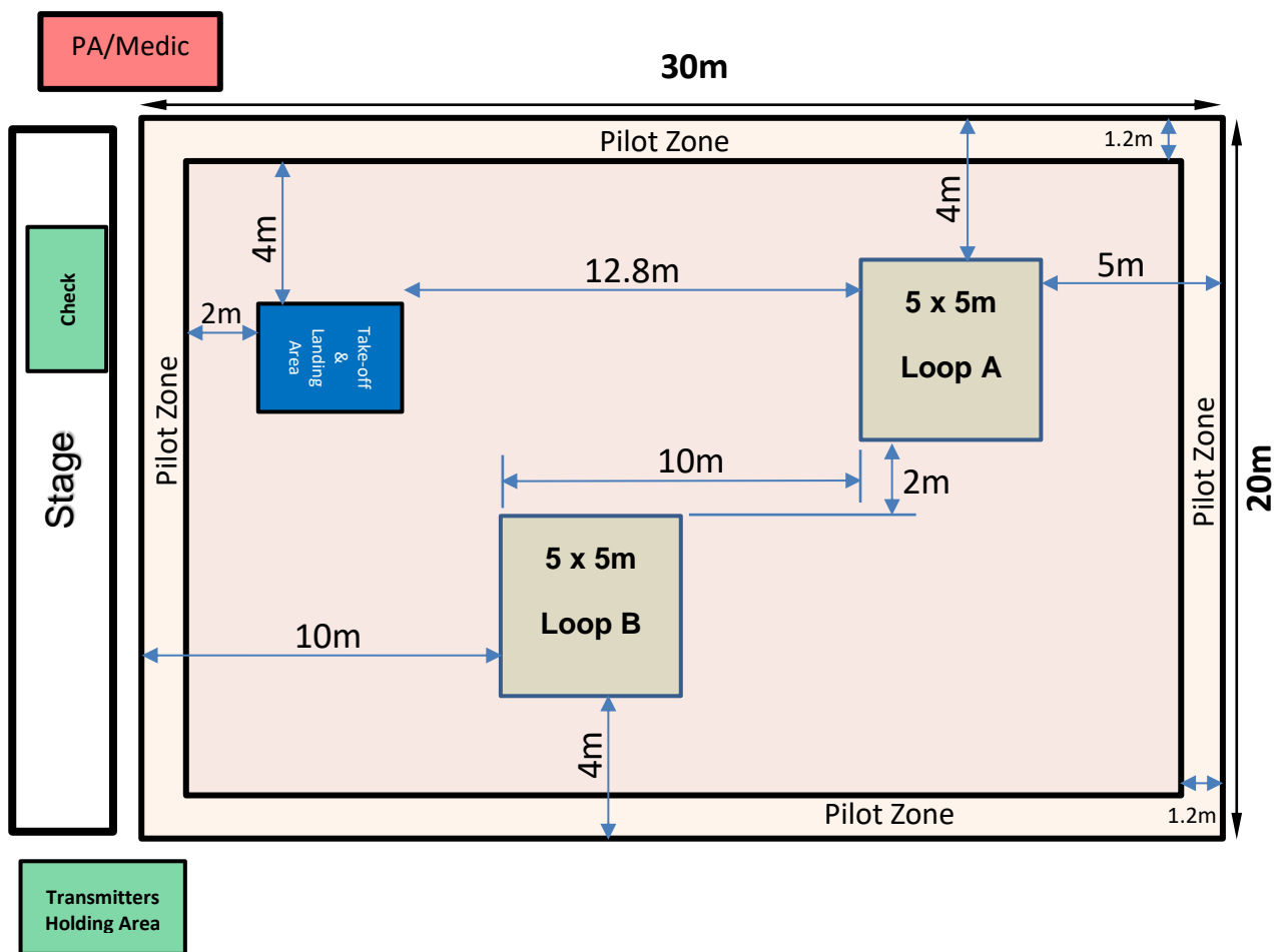
Figure 2 Competition Setup of Category C1 (Plan View)
